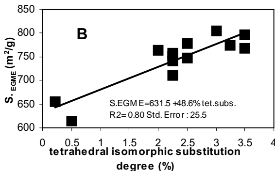
Figure 2c: Linear regression models for S_w as a function of tetrahedral isomorphous substitution degree.
