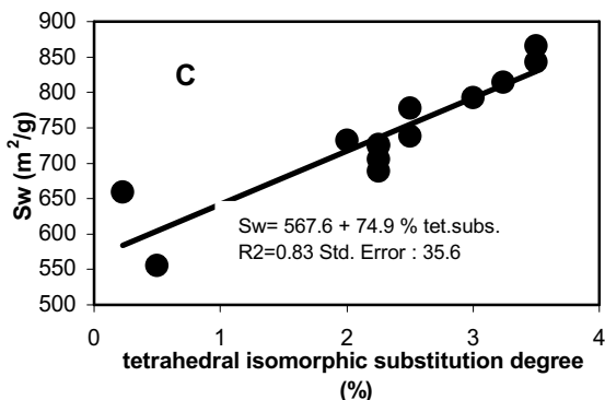
Figure 2b: Linear regression models for S_{EGME} as a function of tetrahedral isomorphous substitution degree.
