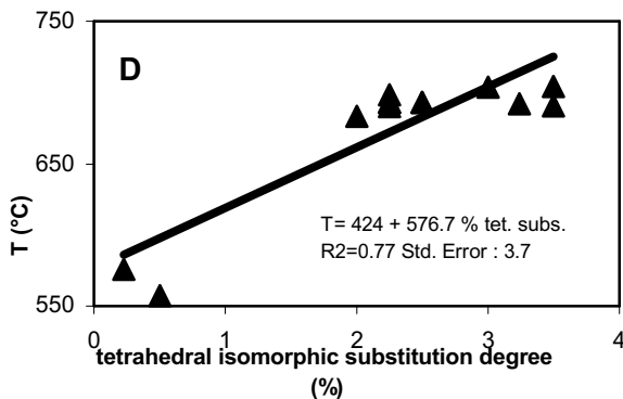
Figure 2d: Linear regression models for T as a function of tetrahedral isomorphous substitution degree.
